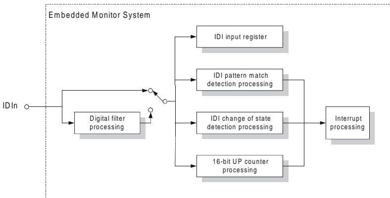
Figure 3.1: PCI-1760 function logic block diagram
