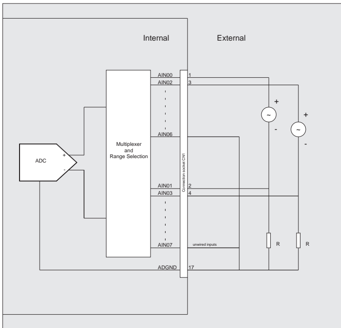
Figure 13.4 Wiring of the A/D inputs (differential)
