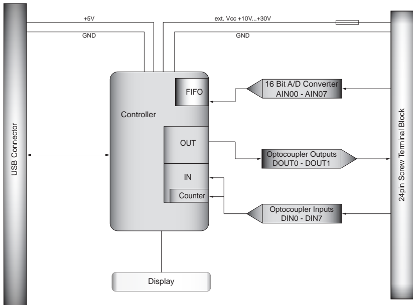
Fig. 3.1 Block diagram EXDUL-381E
