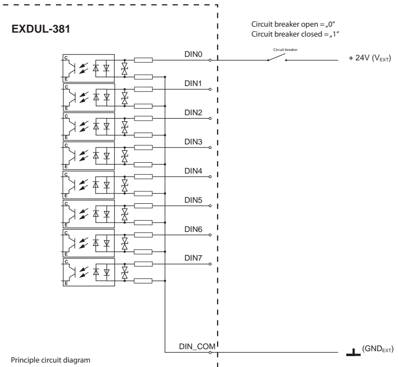
Fig 13.1.1 Wiring of the Optocoupler Inputs
