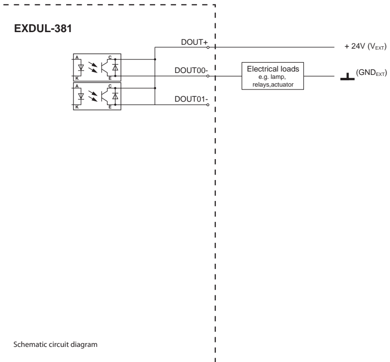
Fig 13.2 Wiring of the optocoupler outputs
