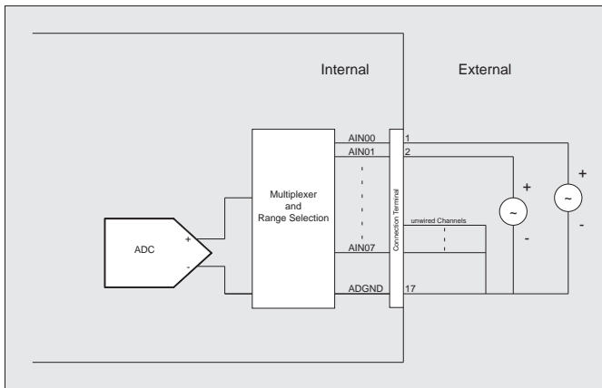
Figure 13.3 Wiring of the A/D inputs (single ended)
