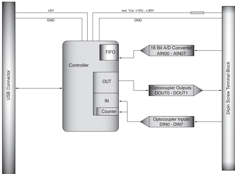
Fig. 3.2 Block diagram EXDUL-381S
