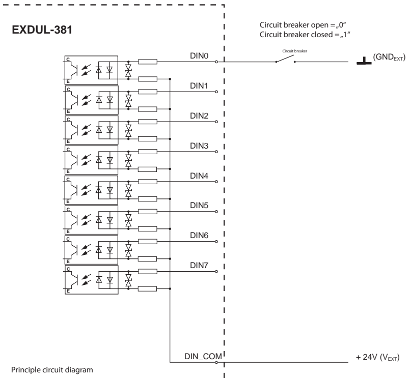
Fig 13.1.2 Wiring of the optocoupler inputs revers
