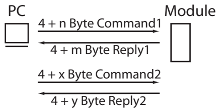
Fig. 10.4 Communication model
