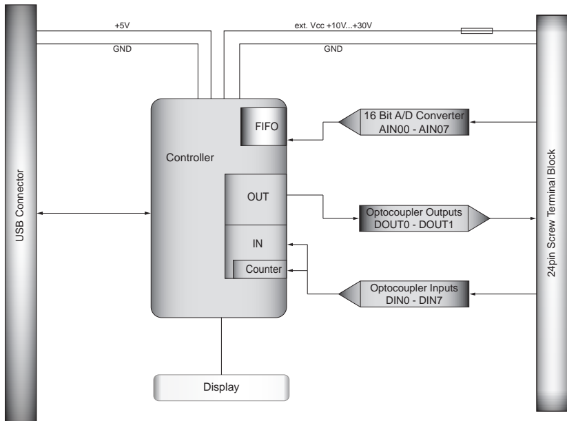
Fig. 3.1 Block diagram EXDUL-381E
